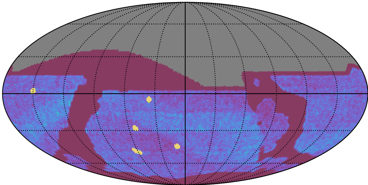
ddf_acor_sf10_lsf15_lsr20_v3.4_10yrs All sky all bands: NVisits
