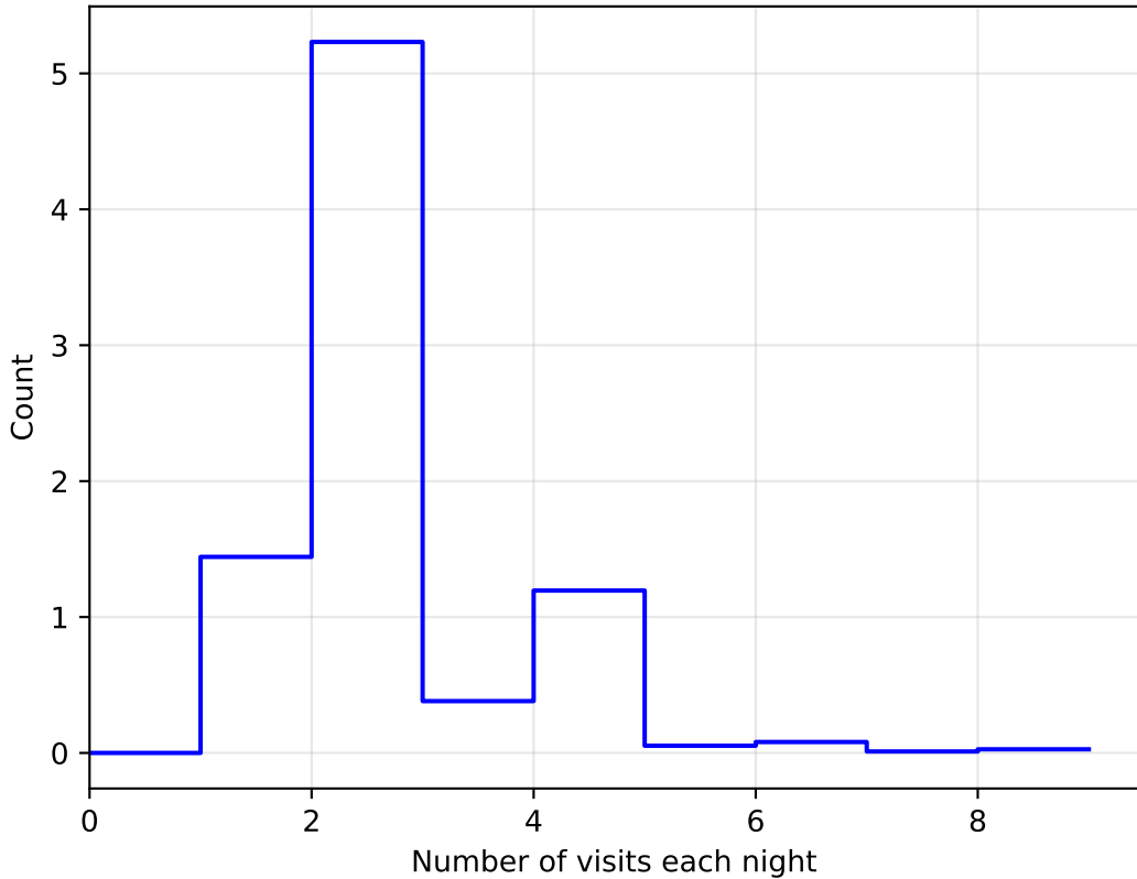
ddf_acor_sf10_lsf15_lsr20_v3.4_10yrs WFD: NVisitsPerNight 1e6
