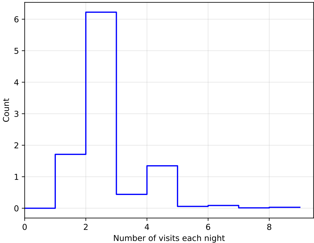
ddf_acor_sf10_lsf15_lsr20_v3.4_10yrs All sky: NVisitsPerNight 1e6
