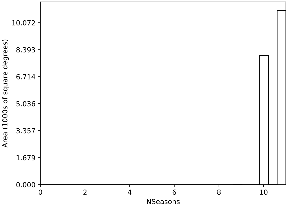
ddf_acor_sf10_lsf15_lsr20_v3.4_10yrs WFD all bands: NSeasons
