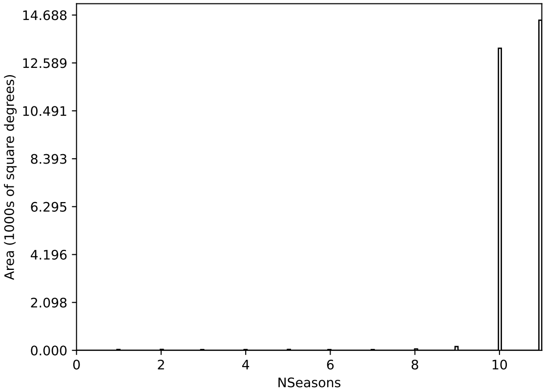
ddf_acor_sf10_lsf15_lsr20_v3.4_10yrs All sky all bands: NSeasons
