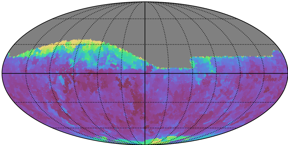
ddf_acor_sf10_lsf15_lsr20_v3.4_10yrs Yr 1 i band: Min seeingEff
