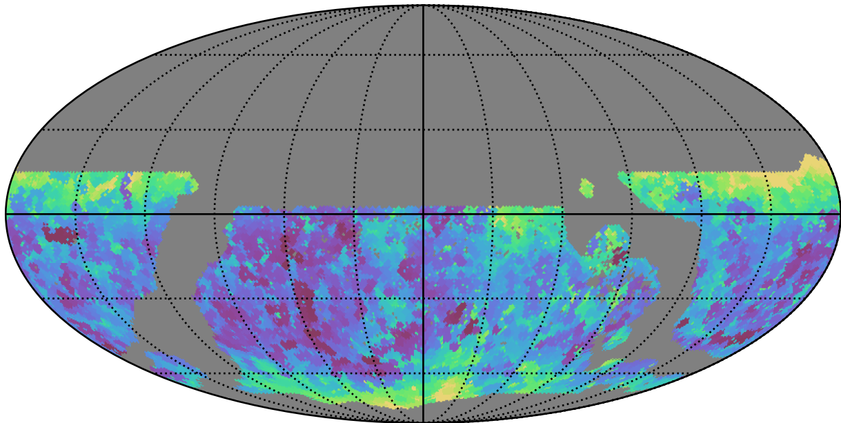
ddf_acor_sf10_lsf15_lsr20_v3.4_10yrs WFD y band: Min seeingEff
