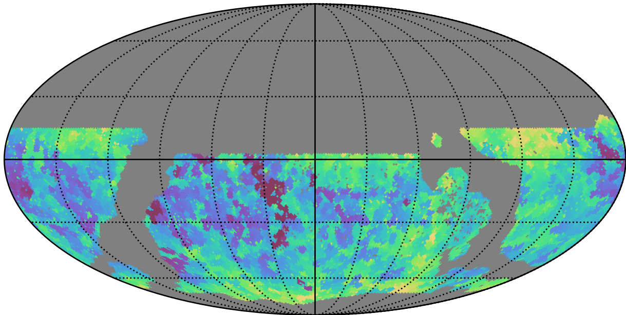
ddf_acor_sf10_lsf15_lsr20_v3.4_10yrs WFD g band: Min seeingEff
