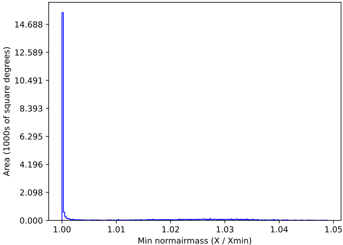
ddf_acor_sf10_lsf15_lsr20_v3.4_10yrs All sky y band: Min normairmass
