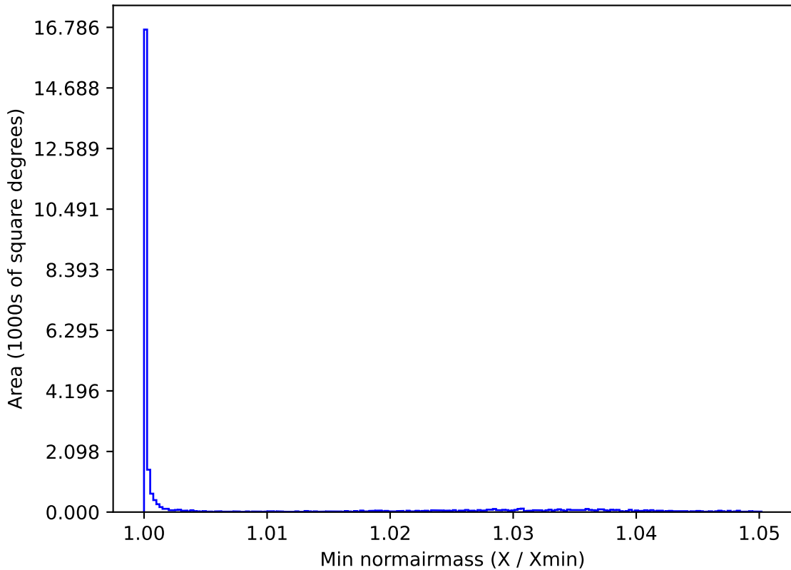
ddf_acor_sf10_lsf15_lsr20_v3.4_10yrs All sky g band: Min normairmass
