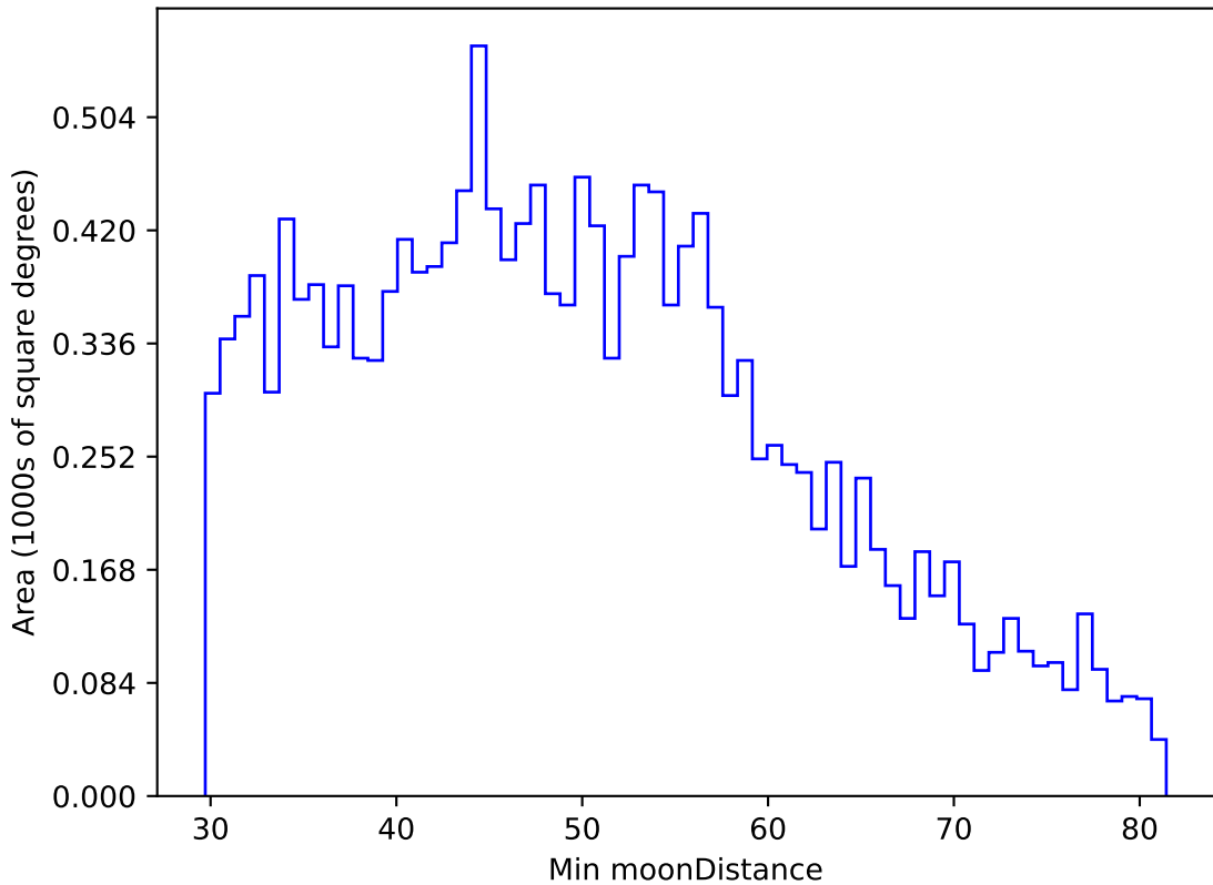
ddf_acor_sf10_lsf15_lsr20_v3.4_10yrs WFD u band: Min moonDistance
