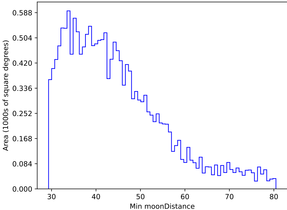
ddf_acor_sf10_lsf15_lsr20_v3.4_10yrs WFD g band: Min moonDistance
