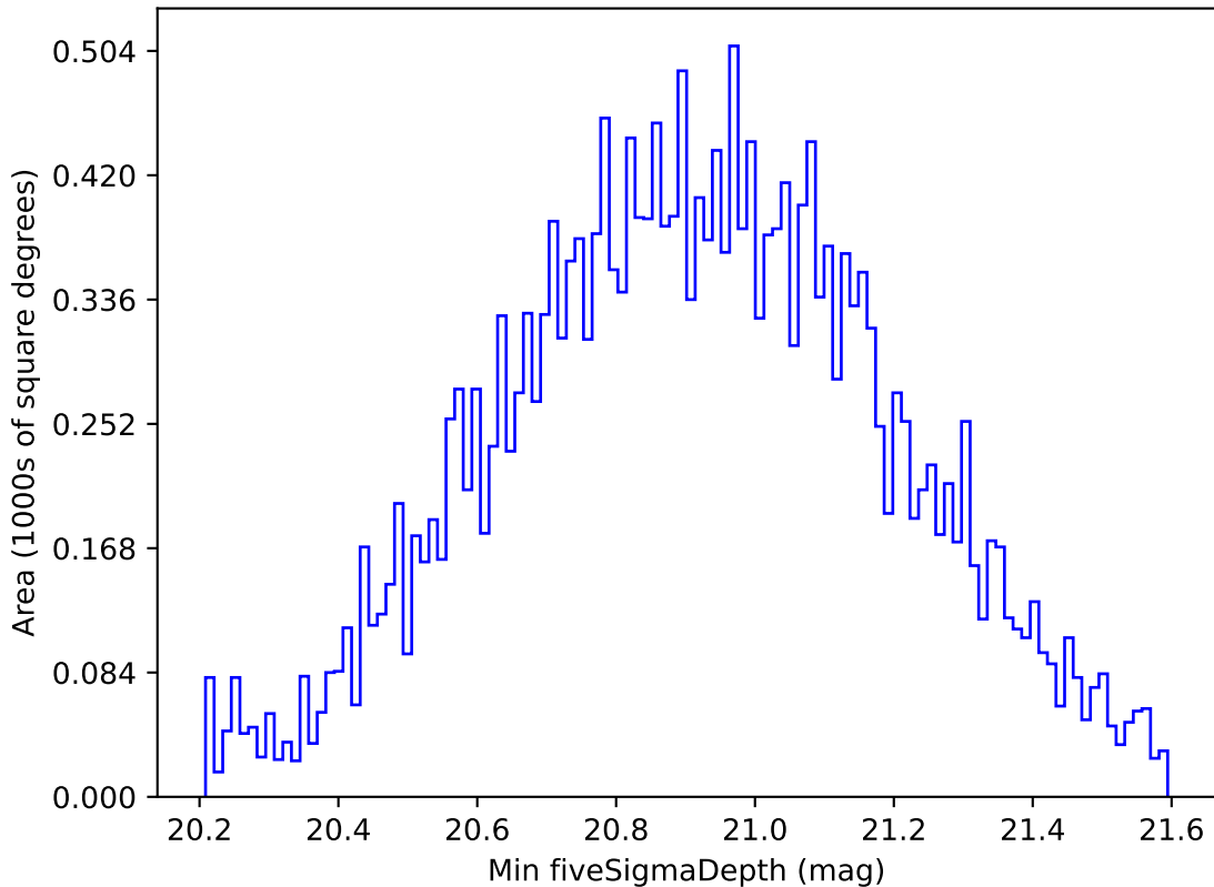
ddf_acor_sf10_lsf15_lsr20_v3.4_10yrs All sky y band: Min fiveSigmaDepth
