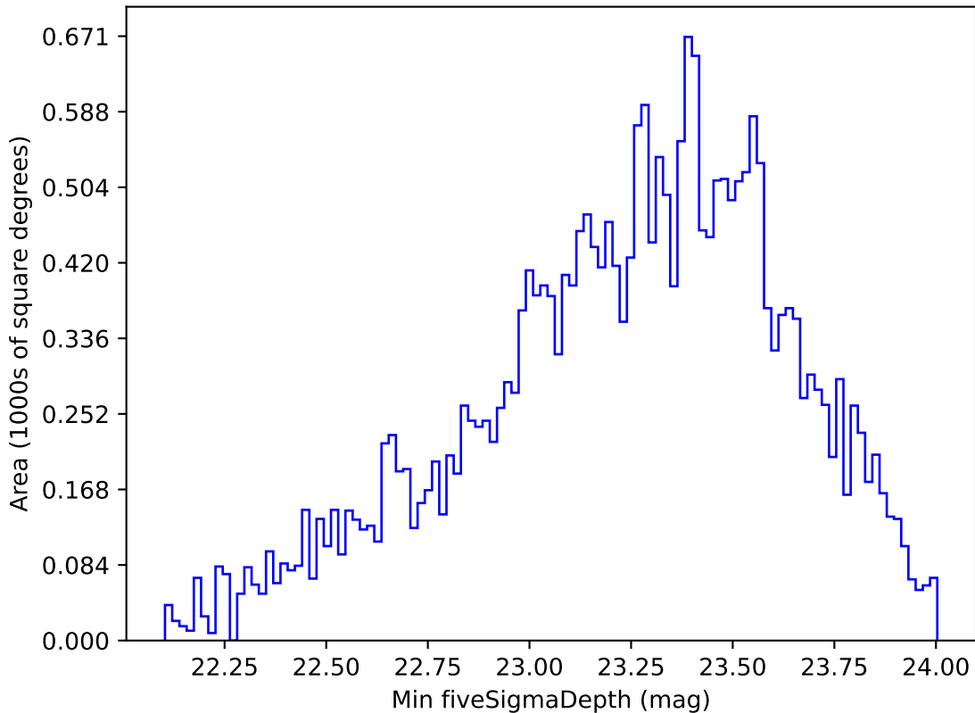
ddf_acor_sf10_lsf15_lsr20_v3.4_10yrs All sky g band: Min fiveSigmaDepth
