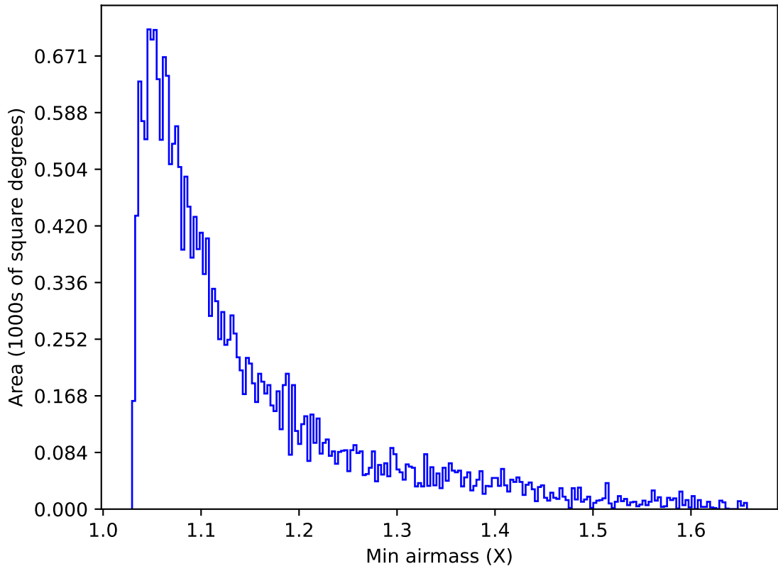
ddf_acor_sf10_ls15_lsr20_v3.4_10yrs Yr 1 u band: Min airmass
