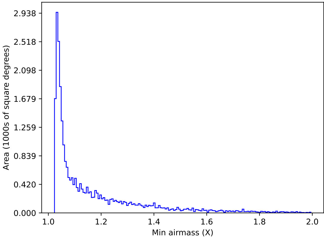
ddf_acor_sf10_lsf15_lsr20_v3.4_10yrs Yr 1 r band: Min airmass
