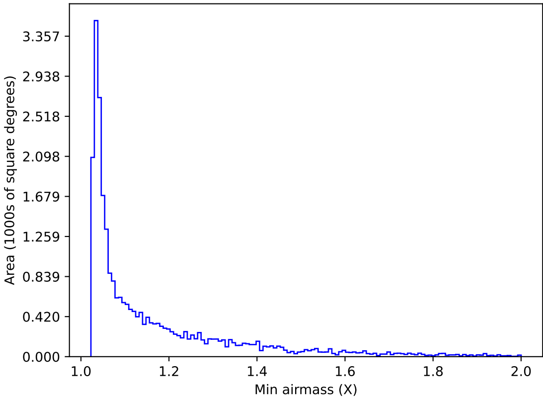
ddf_acor_sf10_lsf15_lsr20_v3.4_10yrs Yr 1 i band: Min airmass
