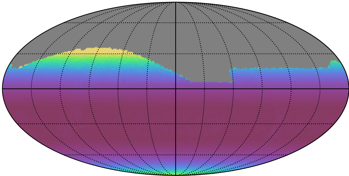
ddf_acor_sf10_lsf15_lsr20_v3.4_10yrs Yr 1 all bands: Min airmass
