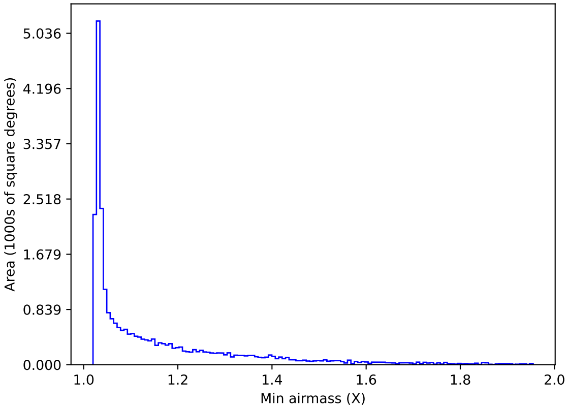
ddf_acor_sf10_lsf15_lsr20_v3.4_10yrs Yr 1 all bands: Min airmass
