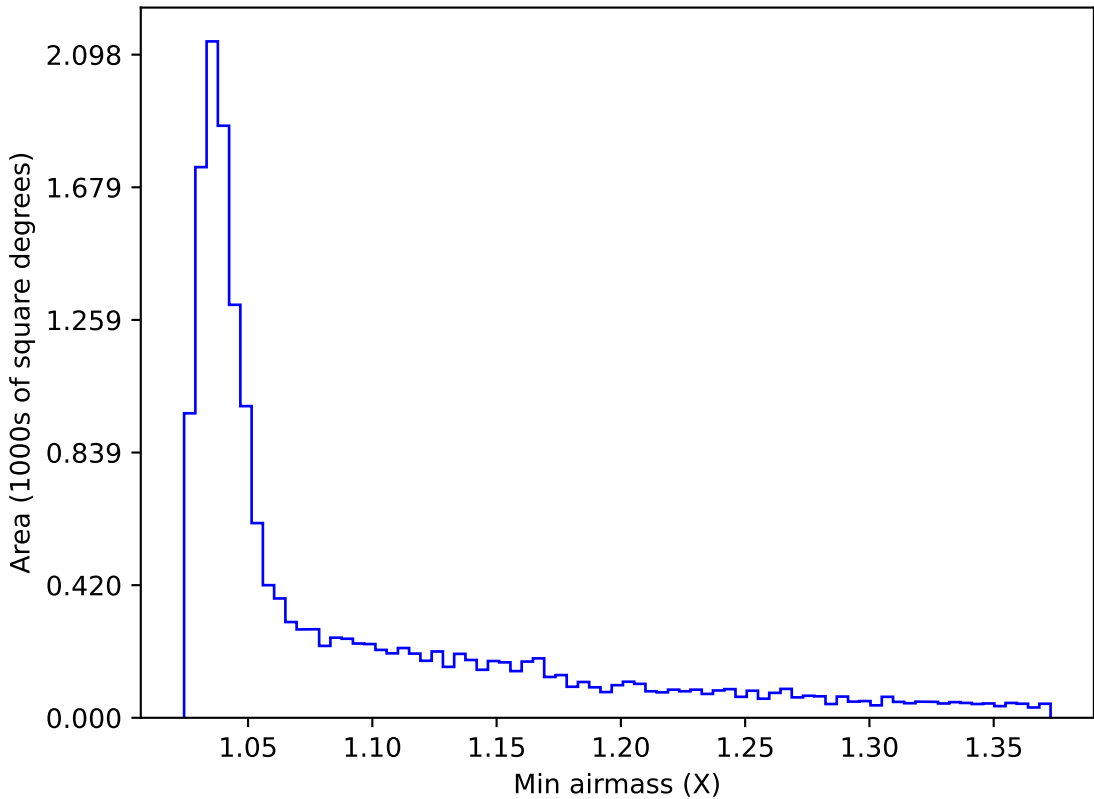
ddf_acor_sf10_lsf15_lsr20_v3.4_10yrs WFD u band: Min airmass
