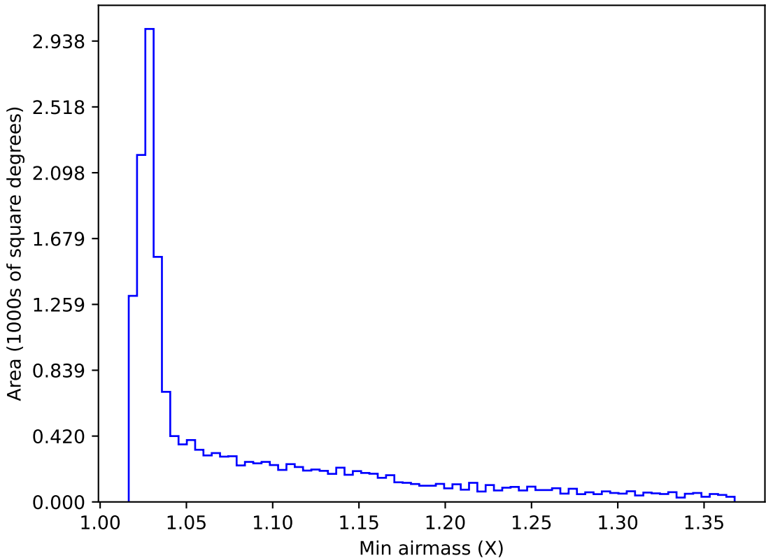
ddf_acor_sf10_lsf15_lsr20_v3.4_10yrs WFD r band: Min airmass
