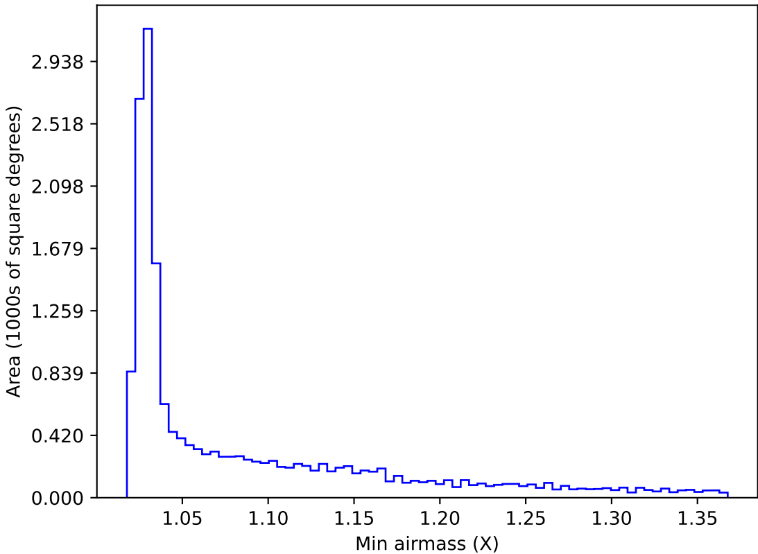
ddf_acor_sf10_lsf15_lsr20_v3.4_10yrs WFD i band: Min airmass
