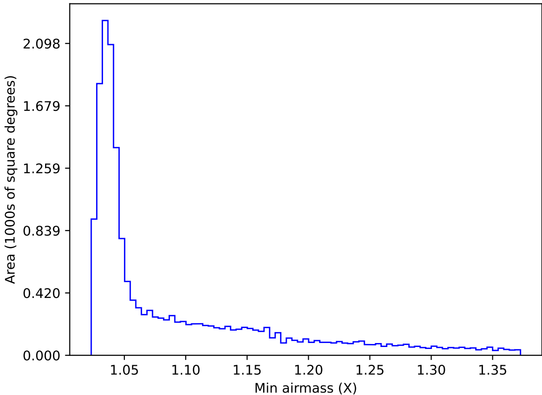
ddf_acor_sf10_lsf15_lsr20_v3.4_10yrs WFD g band: Min airmass
