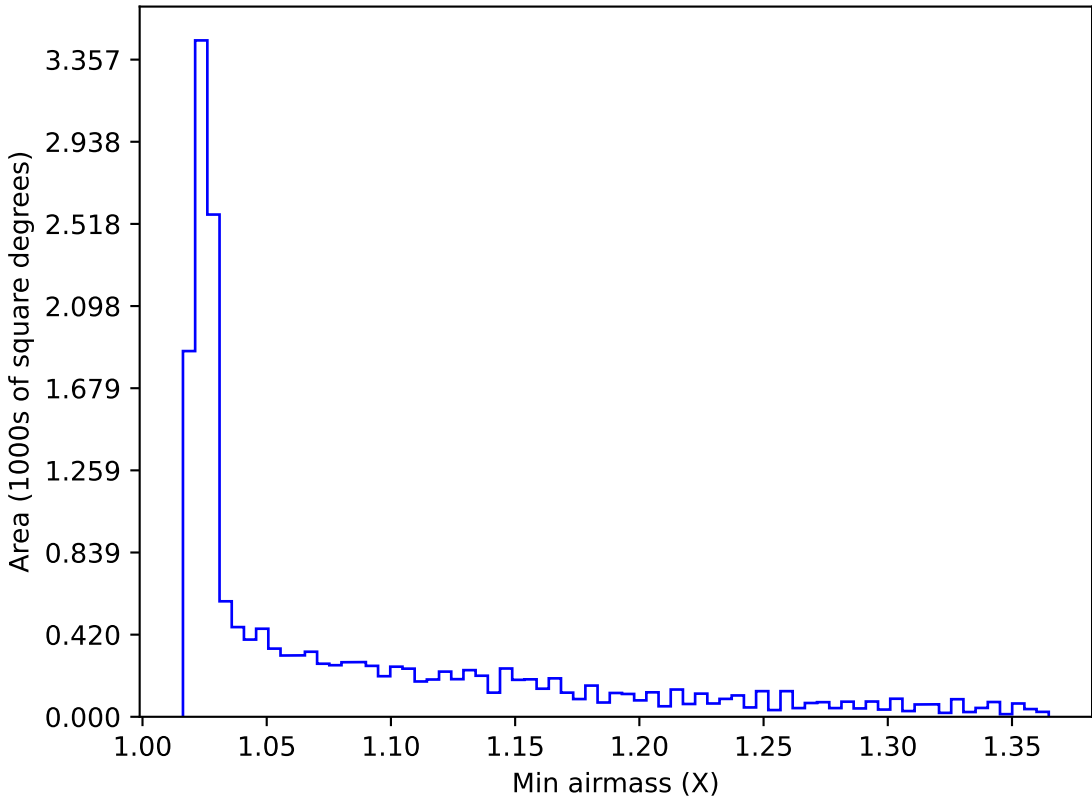
ddf_acor_sf10_lsf15_lsr20_v3.4_10yrs WFD all bands: Min airmass
