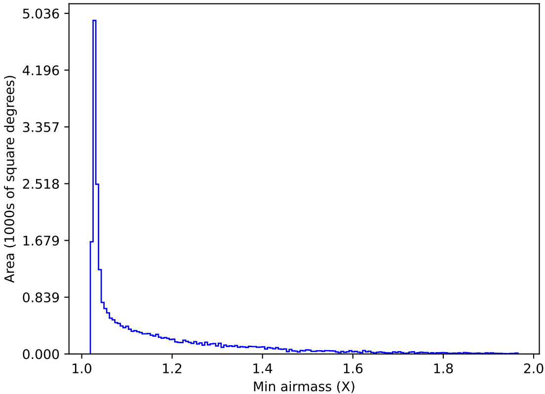
ddf_acor_sf10_lsf15_lsr20_v3.4_10yrs All sky z band: Min airmass
