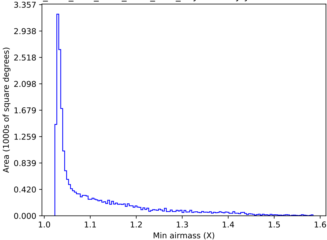
ddf_acor_sf10_lsf15_lsr20_v3.4_10yrs All sky y band: Min airmass
