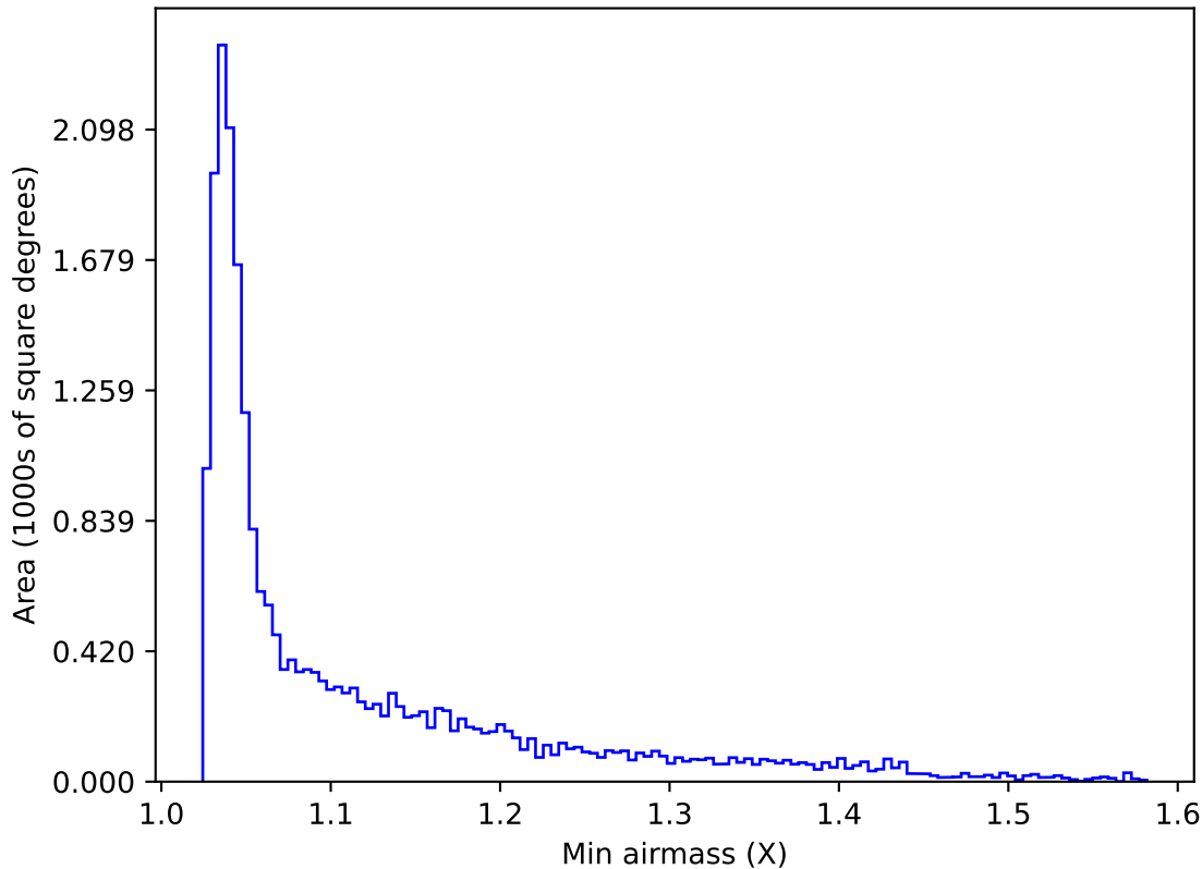
ddf_acor_sf10_lsf15_lsr20_v3.4_10yrs All sky u band: Min airmass
