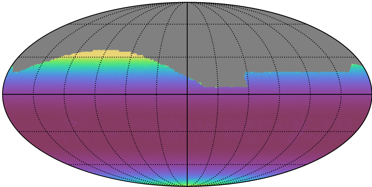
ddf_acor_sf10_lsf15_lsr20_v3.4_10yrs All sky r band: Min airmass
