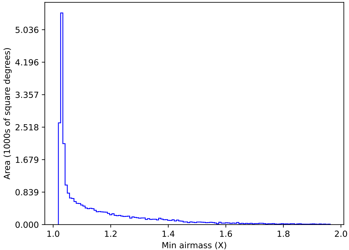
ddf_acor_sf10_lsf15_lsr20_v3.4_10yrs All sky i band: Min airmass
