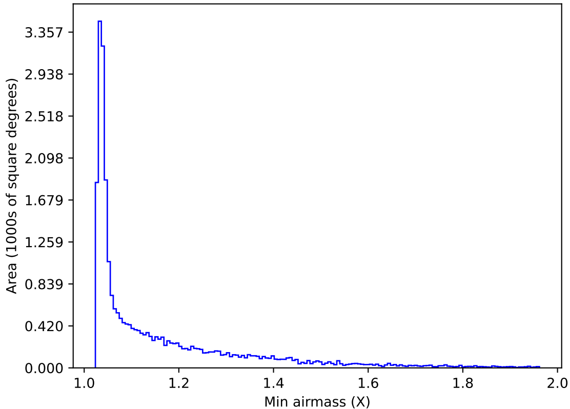
ddf_acor_sf10_lsf15_lsr20_v3.4_10yrs All sky g band: Min airmass
