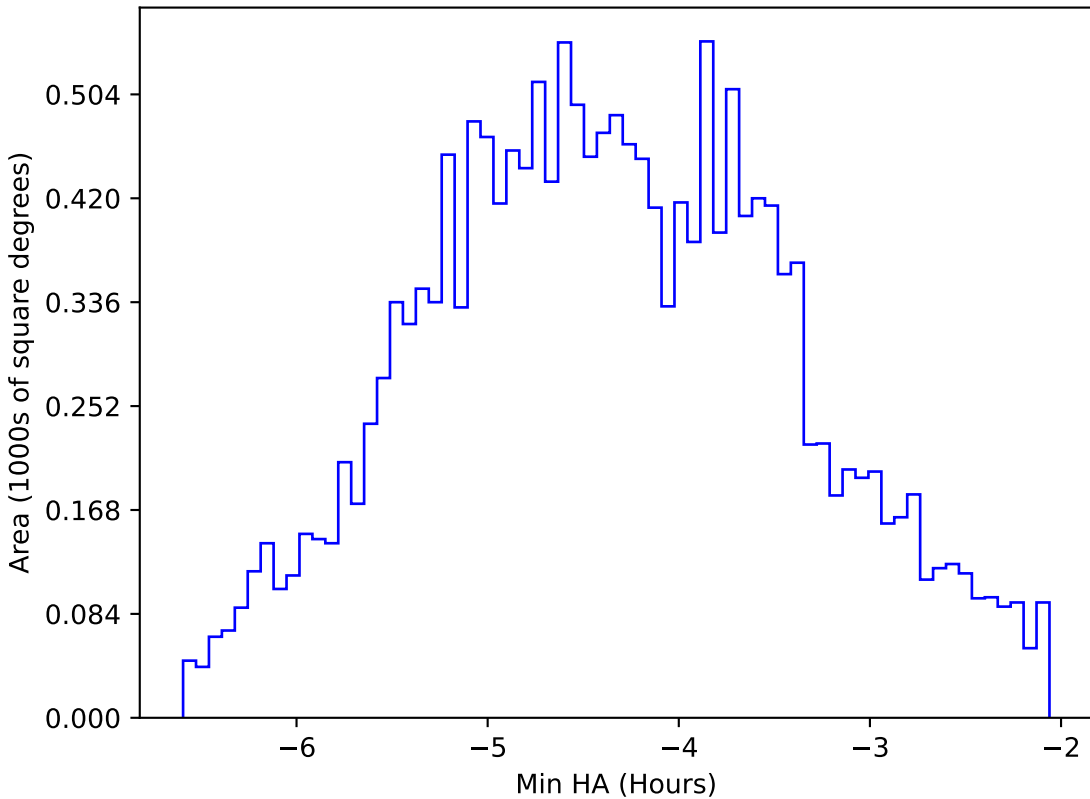
ddf_acor_sf10_lsf15_lsr20_v3.4_10yrs WFD z band: Min HA
