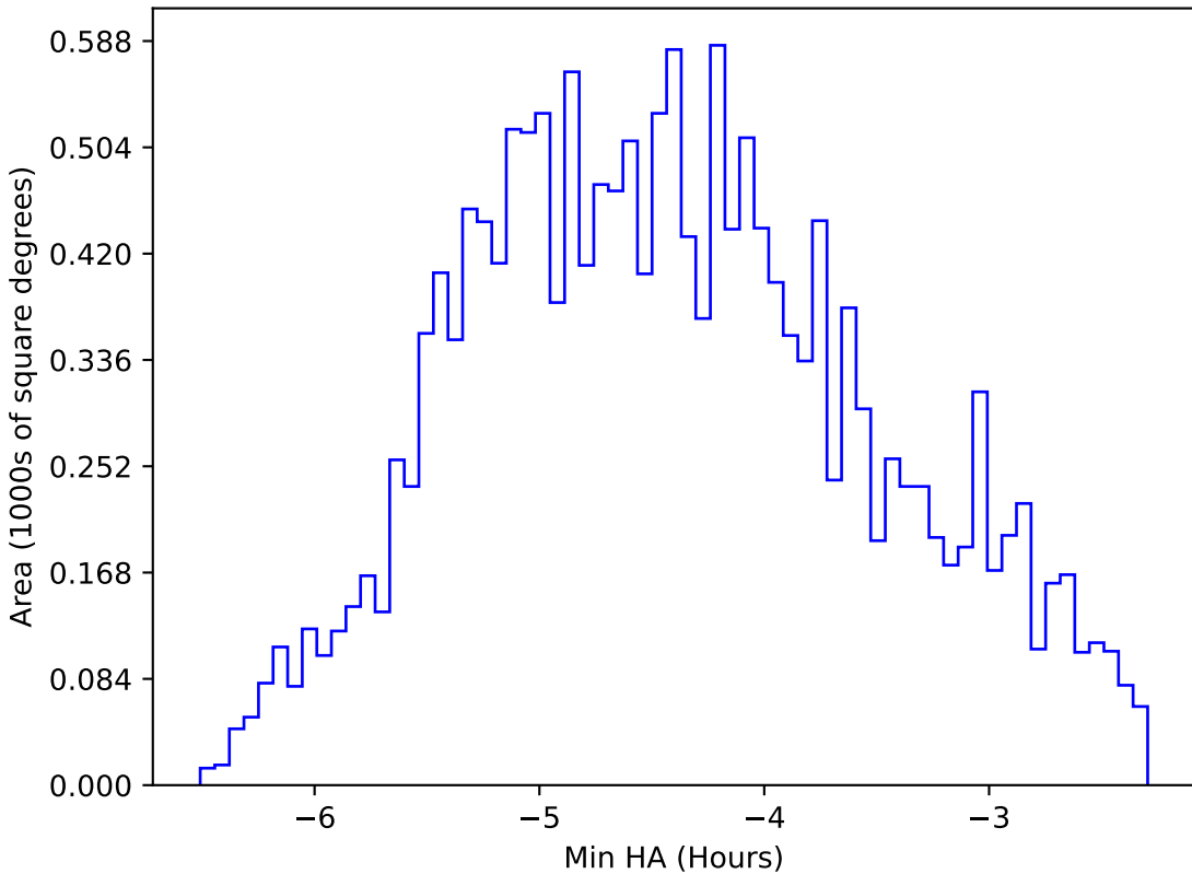
ddf_acor_sf10_lsf15_lsr20_v3.4_10yrs WFD r band: Min HA
