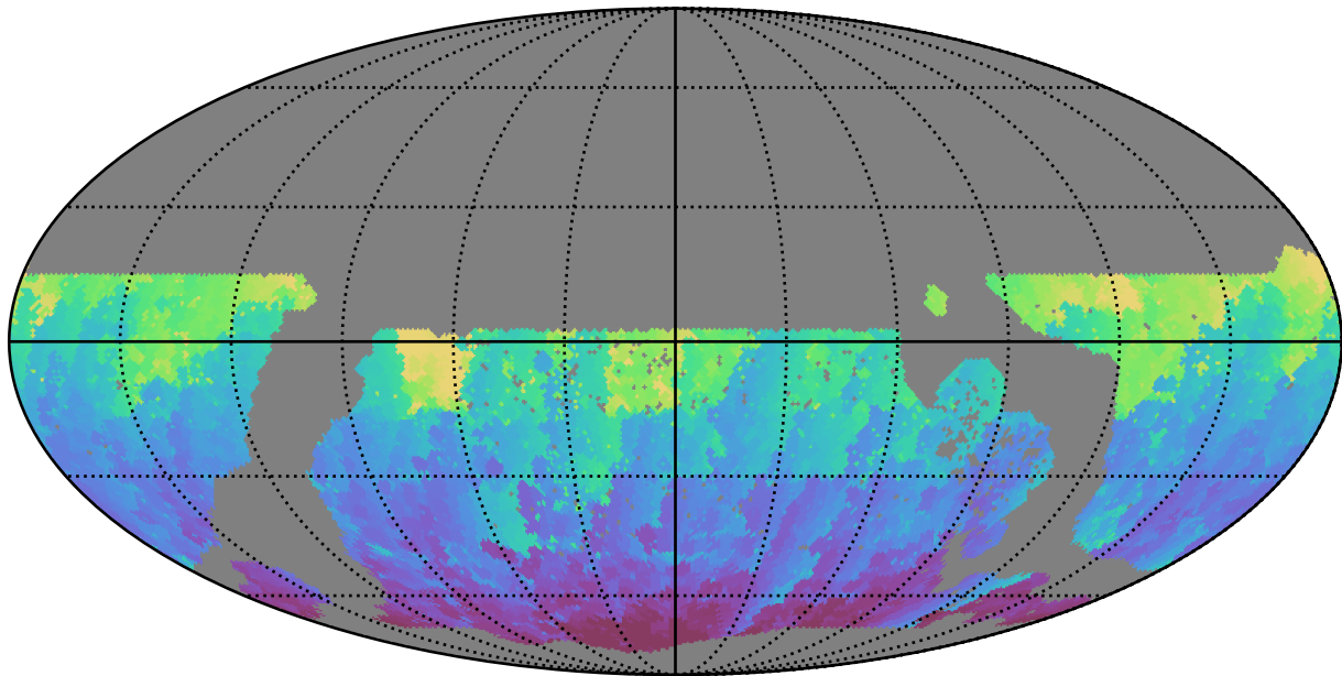
ddf_acor_sf10_lsf15_lsr20_v3.4_10yrs WFD g band: Min HA
