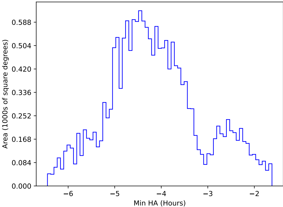
ddf_acor_sf10_lsf15_lsr20_v3.4_10yrs WFD g band: Min HA
