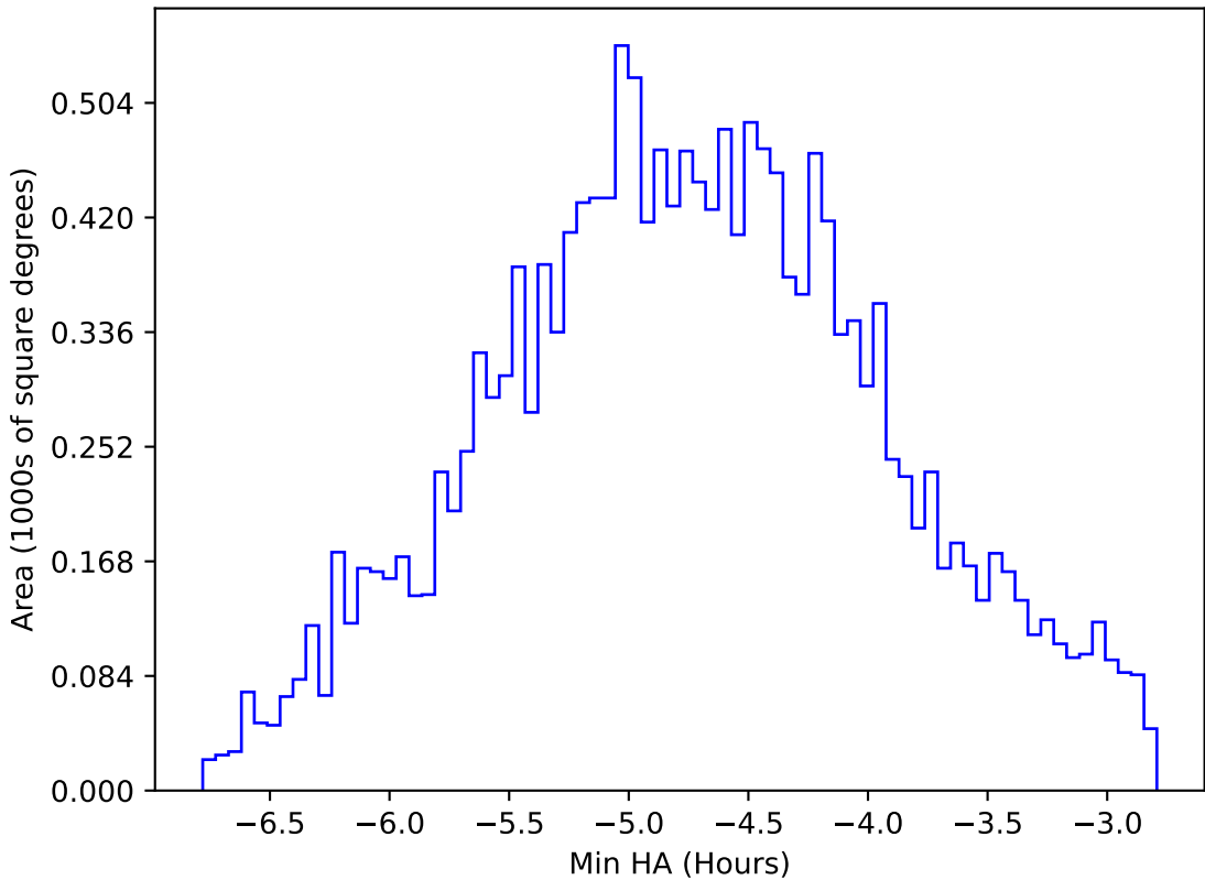
ddf_acor_sf10_ls15_lsr20_v3.4_10yrs WFD all bands: Min HA
