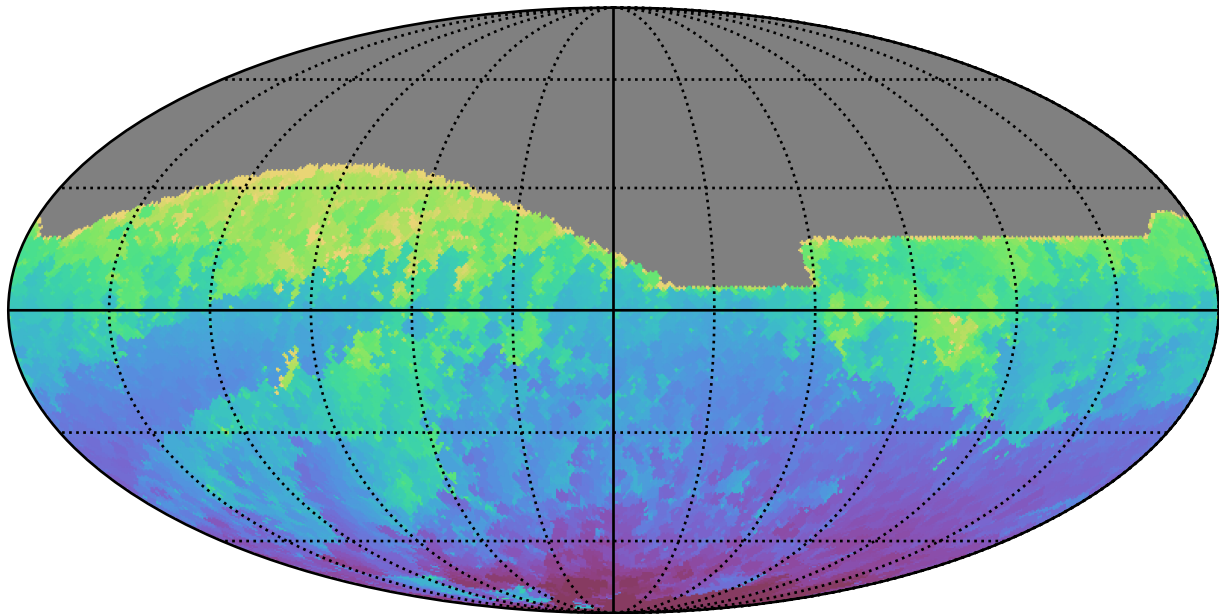
ddf_acor_sf10_lsf15_lsr20_v3.4_10yrs All sky z band: Min HA
