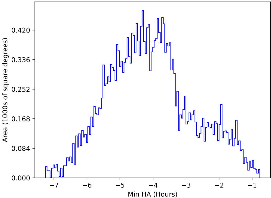
ddf_acor_sf10_lsf15_lsr20_v3.4_10yrs All sky z band: Min HA
