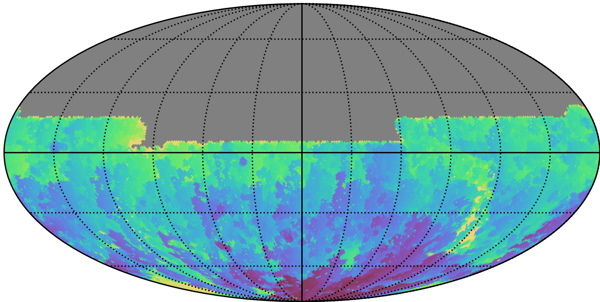
ddf_acor_sf10_lsf15_lsr20_v3.4_10yrs All sky u band: Min HA
