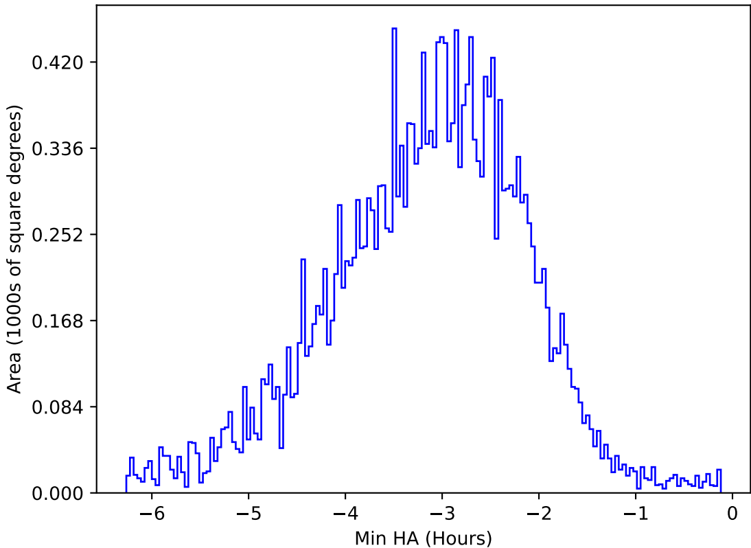
ddf_acor_sf10_ls15_lsr20_v3.4_10yrs All sky u band: Min HA
