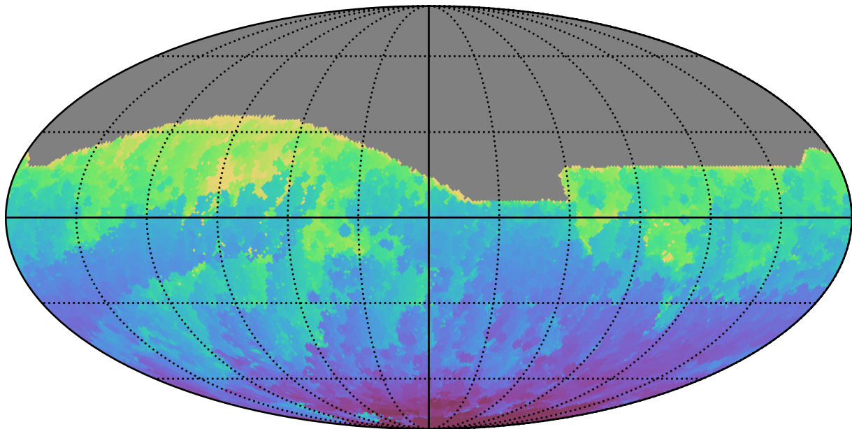
ddf_acor_sf10_lsf15_lsr20_v3.4_10yrs All sky i band: Min HA
