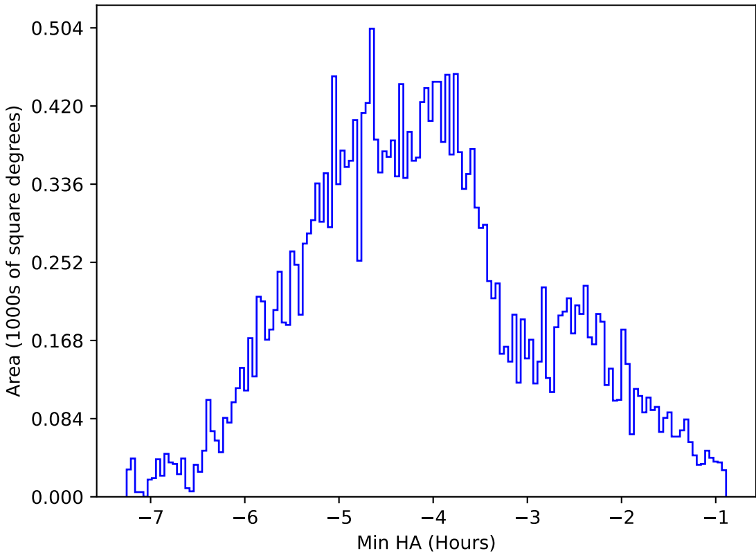
ddf_acor_sf10_ls15_lsr20_v3.4_10yrs All sky i band: Min HA
