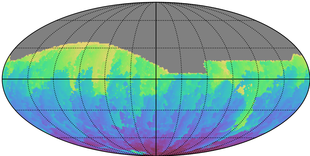
ddf_acor_sf10_lsf15_lsr20_v3.4_10yrs All sky g band: Min HA
