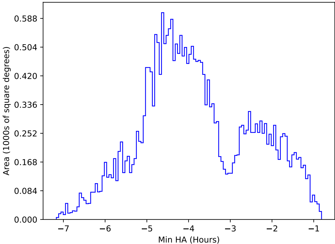
ddf_acor_sf10_ls15_lsr20_v3.4_10yrs All sky g band: Min HA
