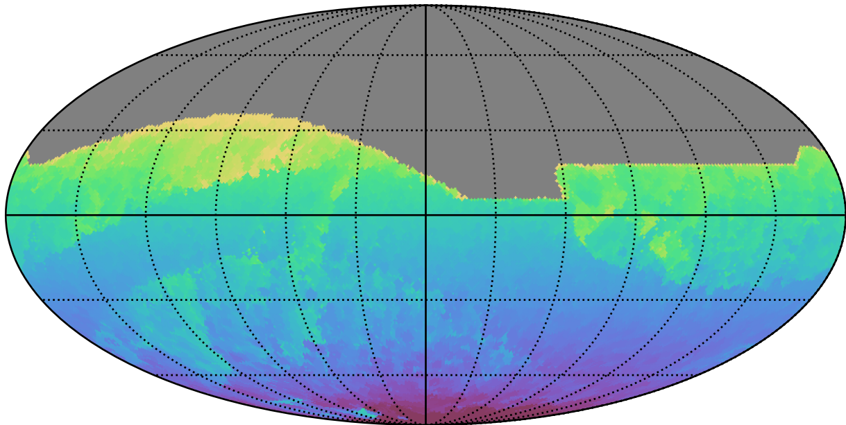
ddf_acor_sf10_lsf15_lsr20_v3.4_10yrs All sky all bands: Min HA
