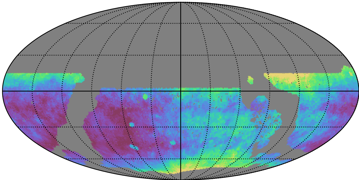
ddf_acor_sf10_lsf15_lsr20_v3.4_10yrs WFD i band: Median seeingEff
