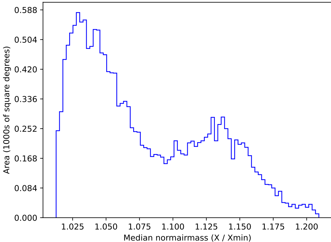
ddf_acor_sf10_lsf15_lsr20_v3.4_10yrs WFD g band: Median normairmass
