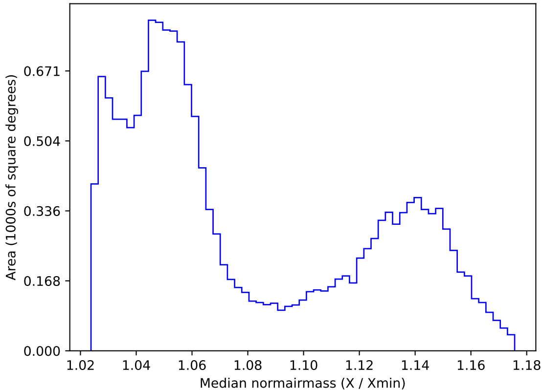
ddf_acor_sf10_lsf15_lsr20_v3.4_10yrs WFD all bands: Median normairmass
