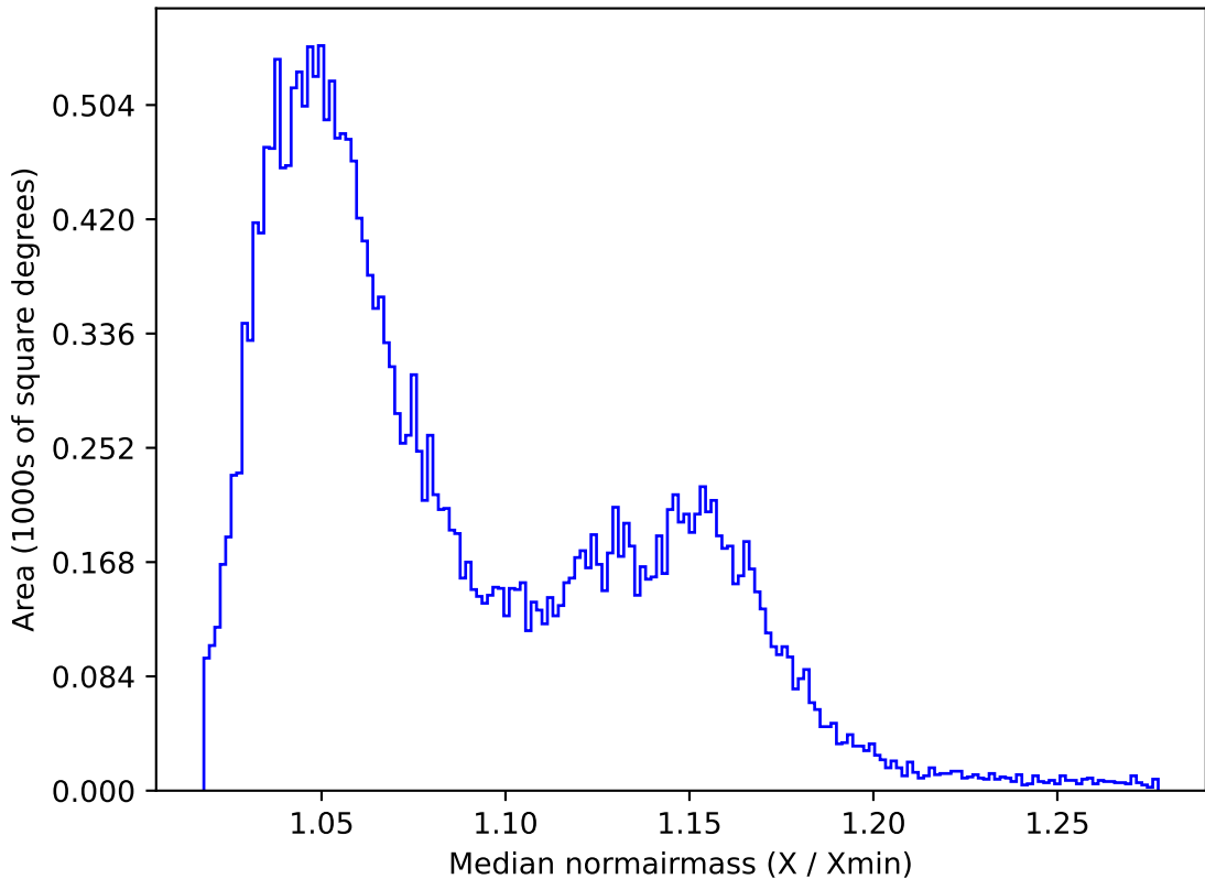
ddf_acor_sf10_ls15_lsr20_v3.4_10yrs All sky z band: Median normairmass
