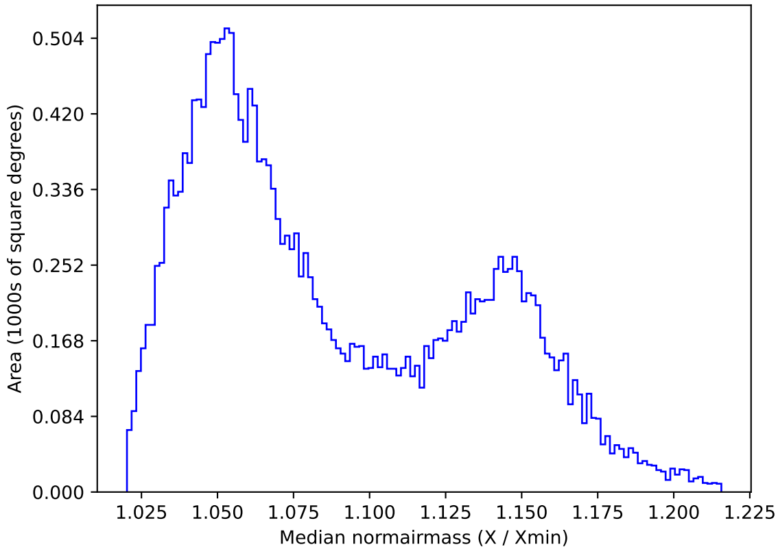
ddf_acor_sf10_ls15_lsr20_v3.4_10yrs All sky y band: Median normairmass
