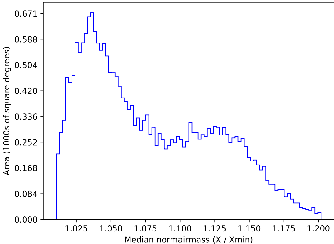
ddf_acor_sf10_ls15_lsr20_v3.4_10yrs All sky u band: Median normairmass
